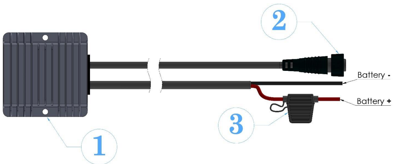
1. DC stabilizer 2. power connector 3. fuse (10 A)
